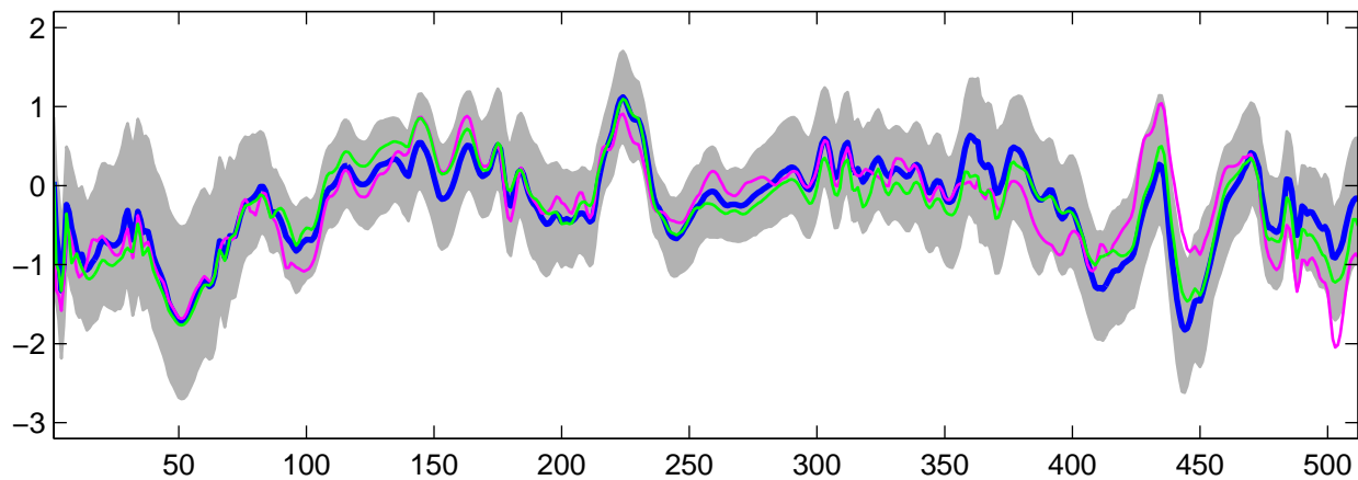
Estimated U_{22}(t) using G-WFMM: t_3 data, run 3
