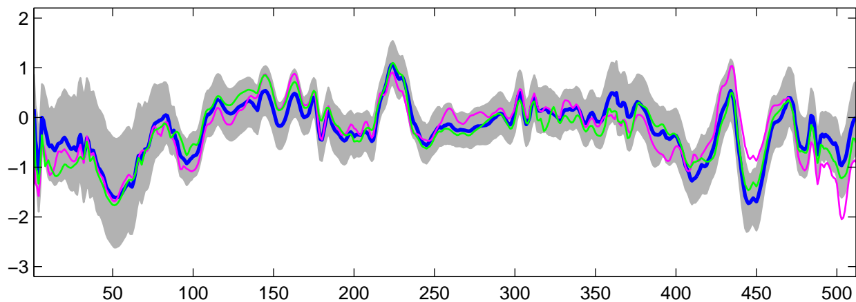
Estimated U_{22}(t) using R-WFMM: t_3 data, run 3
