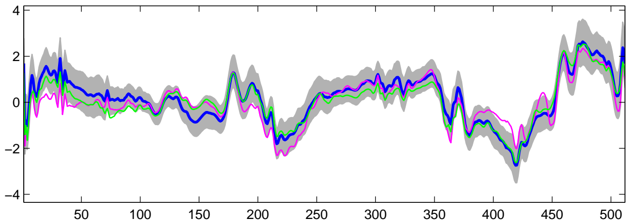
Estimated U_{23}(t) using R-WFMM: DE data, run 3
