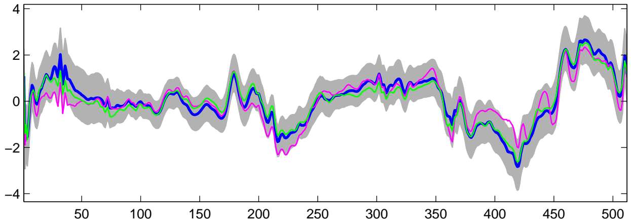
Estimated U_{23}(t) using G-WFMM: DE data, run 3
