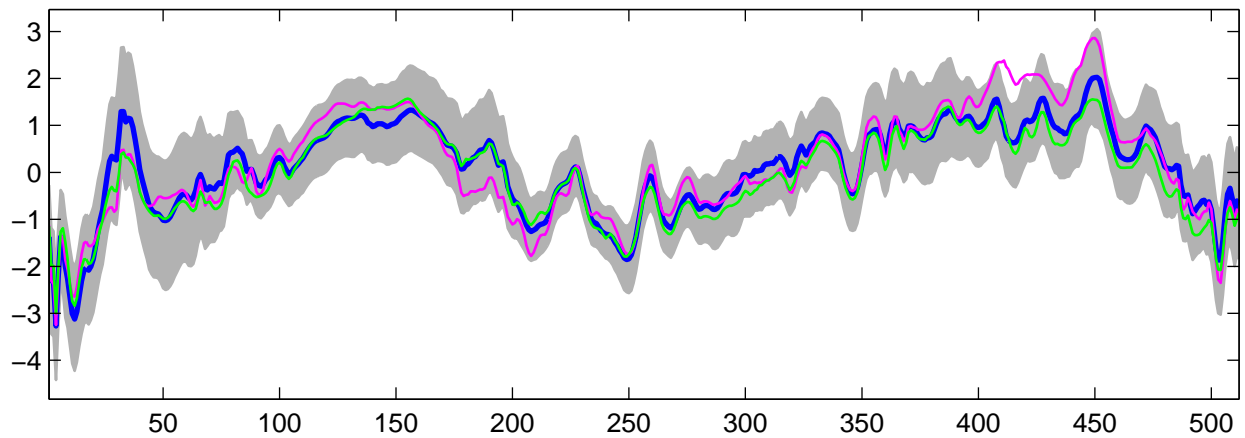
Estimated U_{23}(t) using R-WFMM: Normal data, run 3
