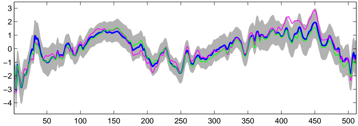
Estimated U_{23}(t) using G-WFMM: Normal data, run 3
