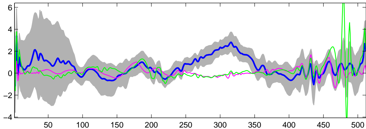
Estimated U_{23}(t) using G-WFMM: t_1 data, run 3
