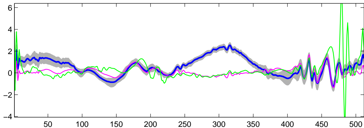
Estimated U_{23}(t) using R-WFMM: t_1 data, run 3
