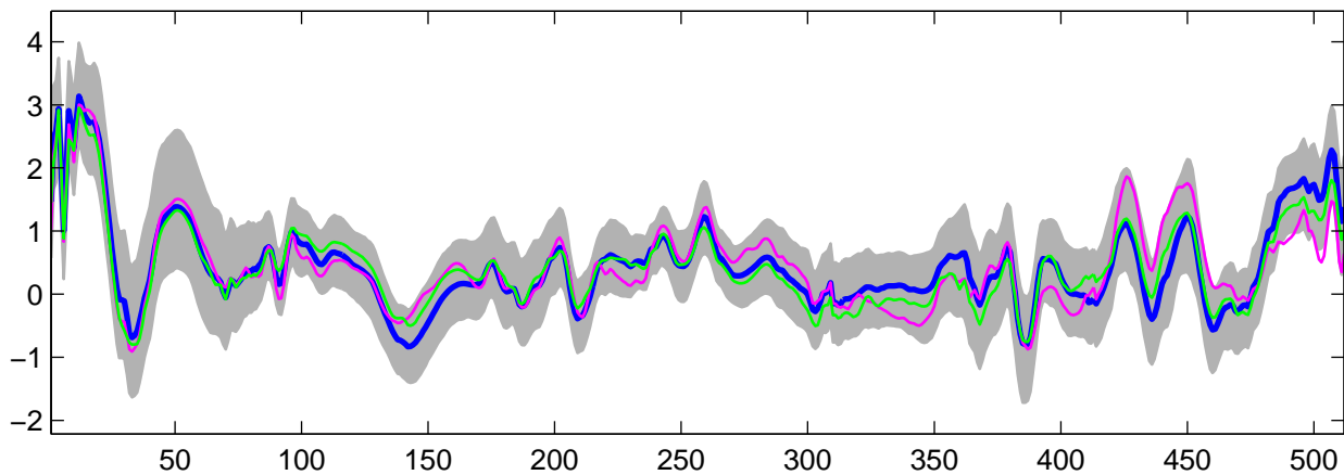
Estimated U_{23}(t) using G-WFMM: t_3 data, run 3
