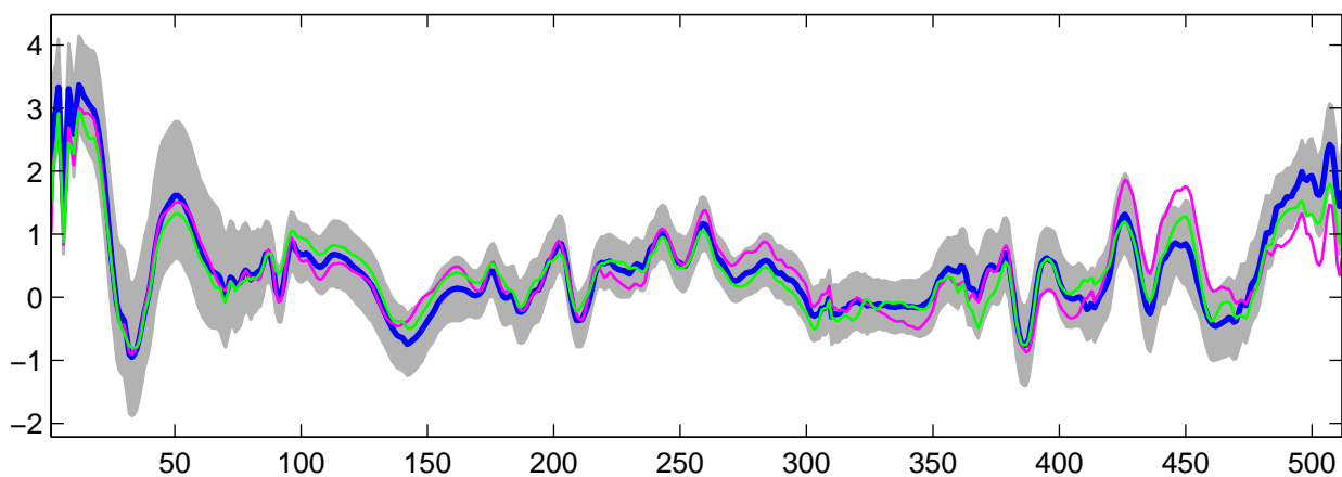
Estimated U_{23}(t) using R-WFMM: t_3 data, run 3
