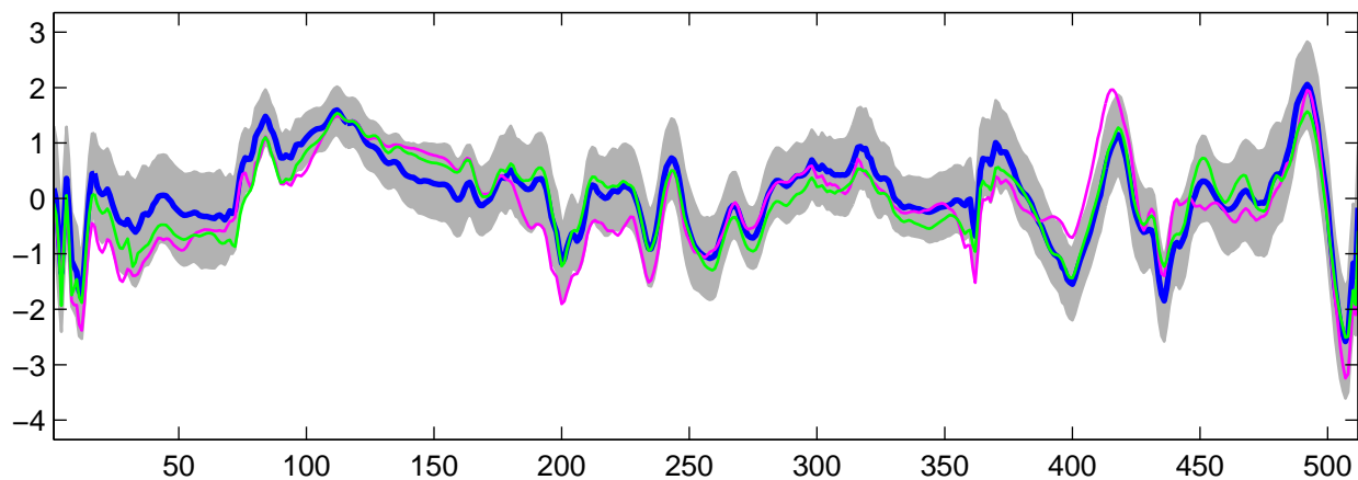
Estimated U_{24}(t) using R-WFMM: DE data, run 3
