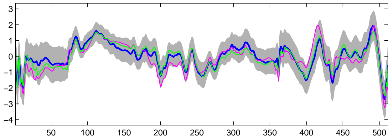
Estimated U_{24}(t) using G-WFMM: DE data, run 3
