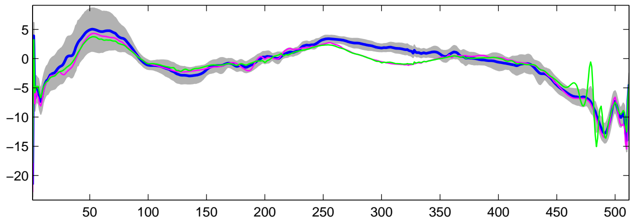
Estimated U_{24}(t) using G-WFMM: t_1 data, run 3
