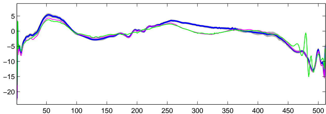
Estimated U_{24}(t) using R-WFMM: t_1 data, run 3
