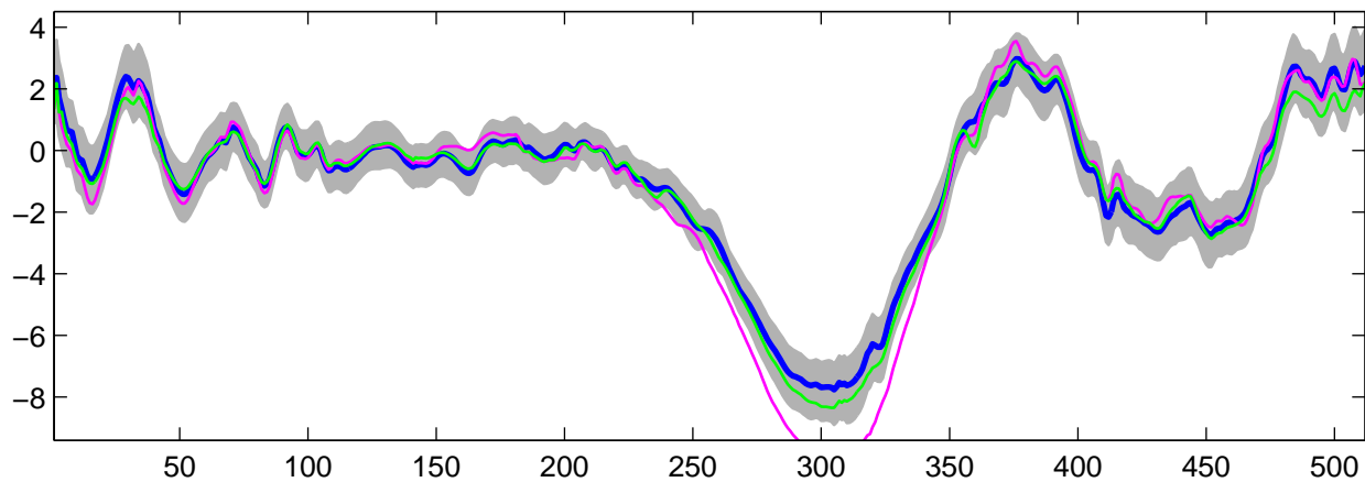
Estimated U_{24}(t) using G-WFMM: t_2 data, run 3
