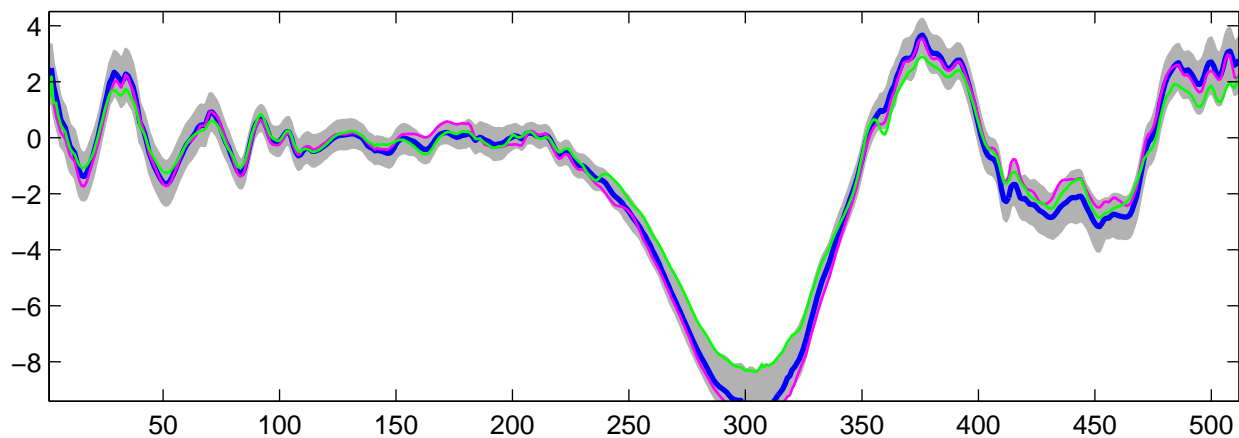
Estimated U_{24}(t) using R-WFMM: t_2 data, run 3
