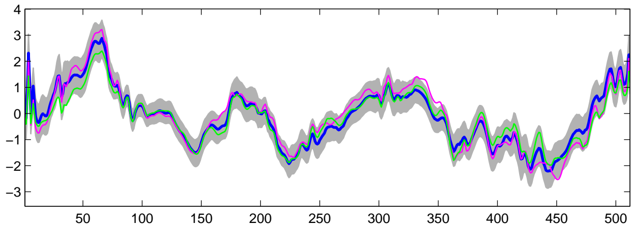
Estimated U_{25}(t) using R-WFMM: DE data, run 3
