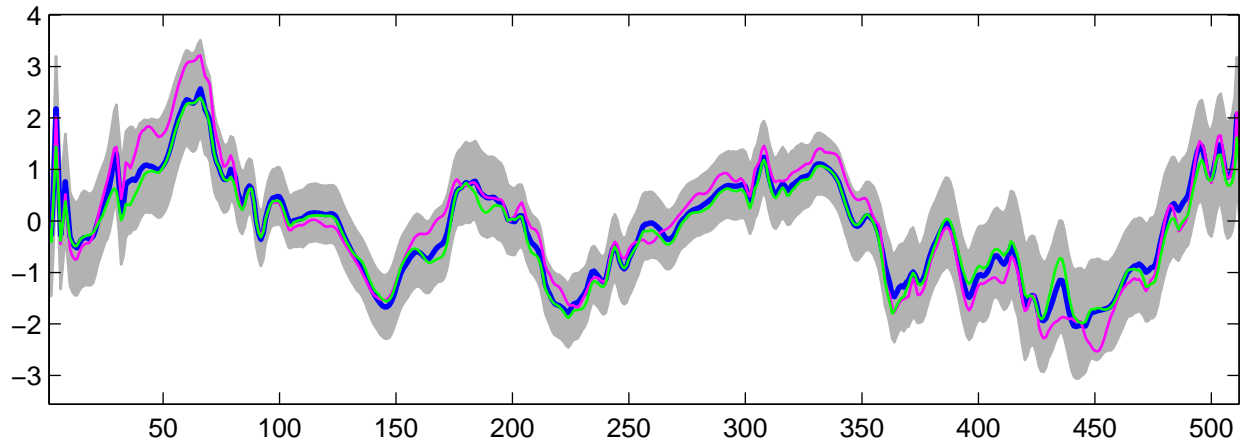
Estimated U_{25}(t) using G-WFMM: DE data, run 3
