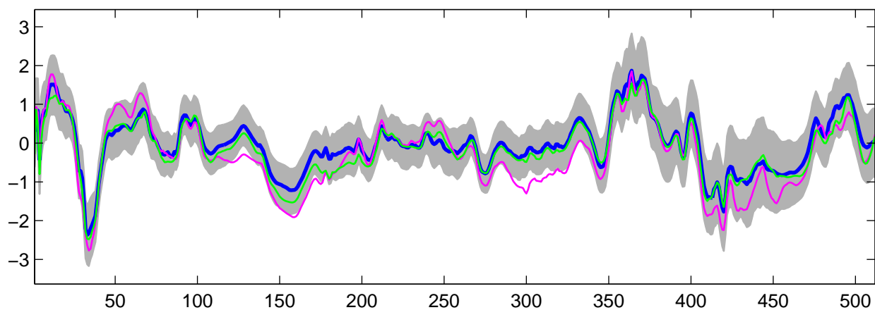
Estimated U_{25}(t) using R-WFMM: Normal data, run 3
