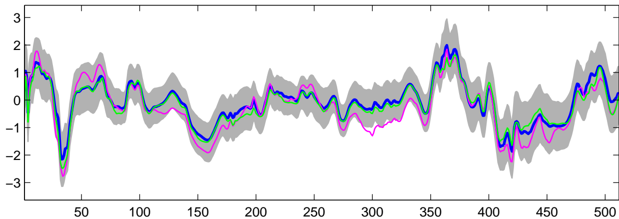
Estimated U_{25}(t) using G-WFMM: Normal data, run 3
