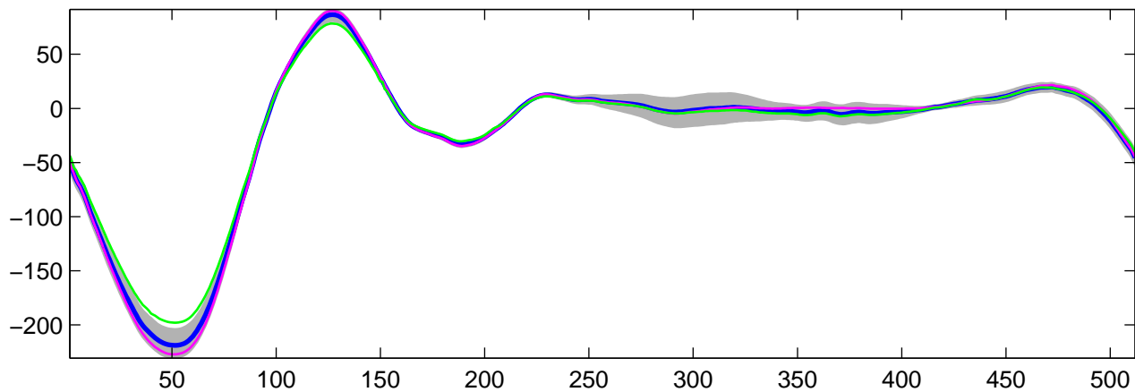
Estimated U_{25}(t) using G-WFMM: t_1 data, run 3
