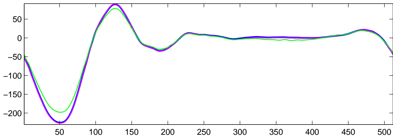
Estimated U_{25}(t) using R-WFMM: t_1 data, run 3
