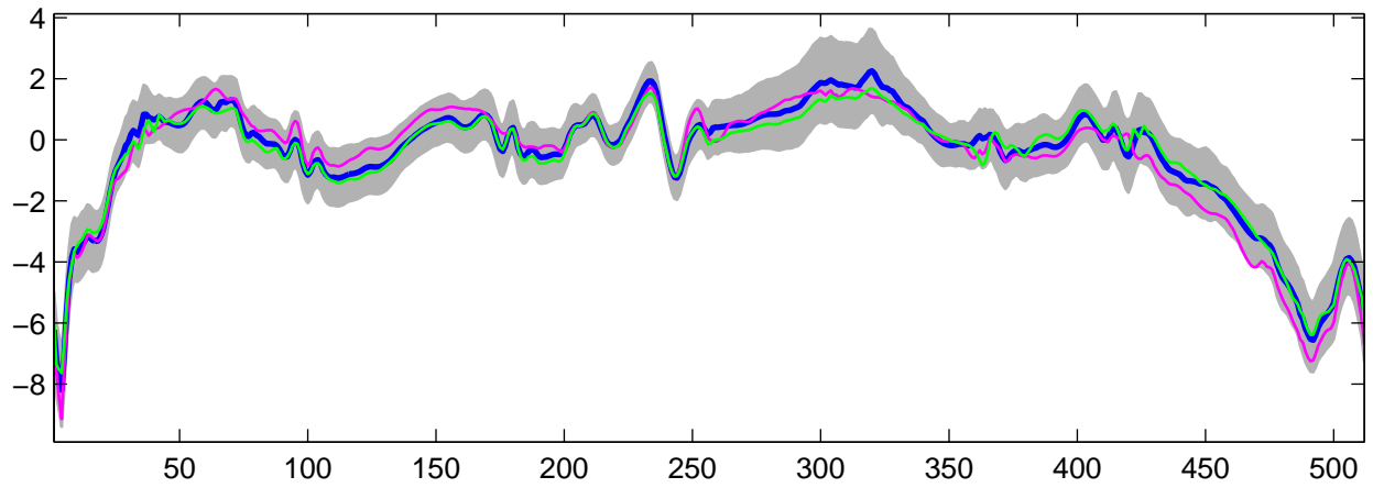
Estimated U_{25}(t) using G-WFMM: t_2 data, run 3
