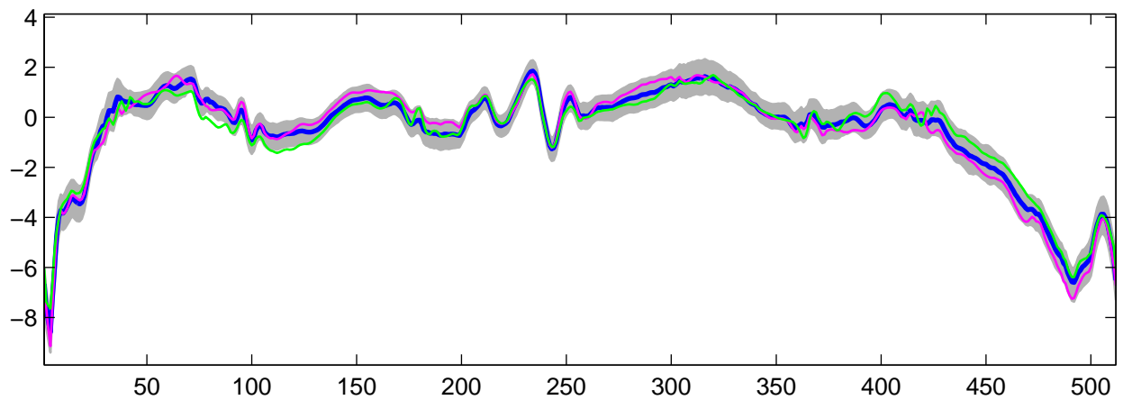
Estimated U_{25}(t) using R-WFMM: t_2 data, run 3
