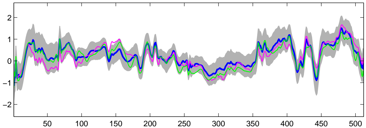
Estimated U_{25}(t) using R-WFMM: t_3 data, run 3
