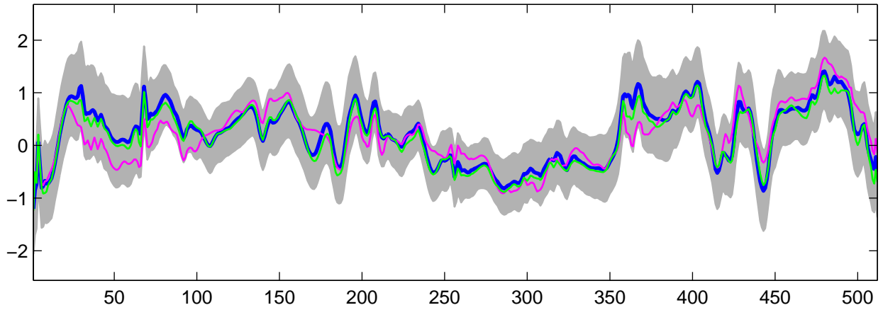
Estimated U_{25}(t) using G-WFMM: t_3 data, run 3
