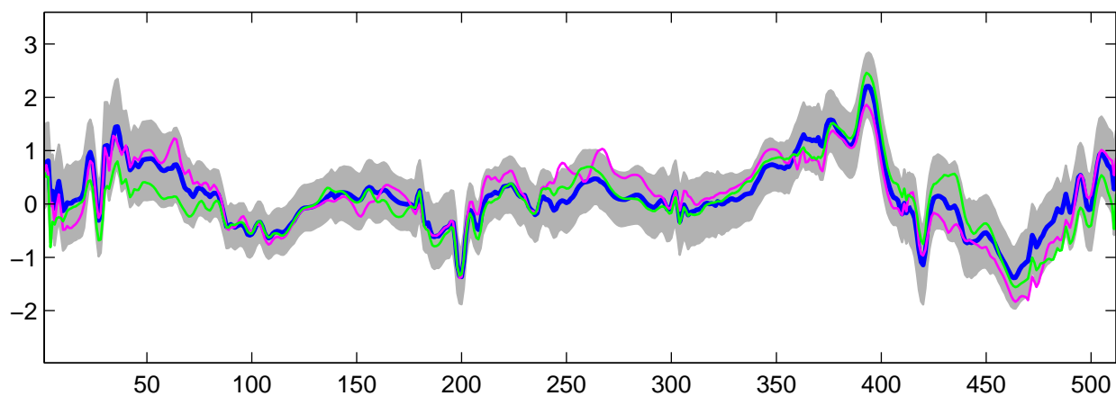
Estimated U_{26}(t) using R-WFMM: DE data, run 3
