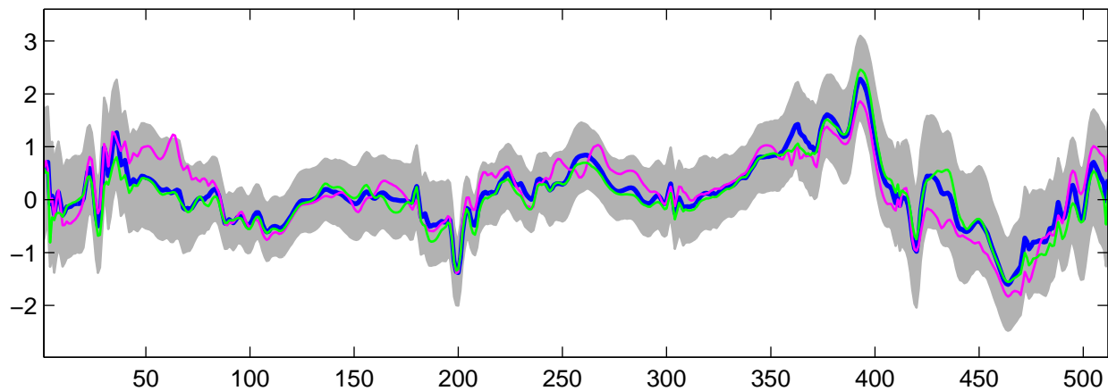
Estimated U_{26}(t) using G-WFMM: DE data, run 3
