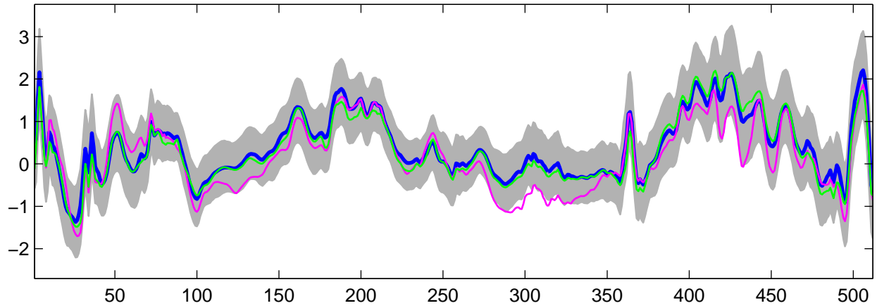
Estimated U_{26}(t) using G-WFMM: Normal data, run 3
