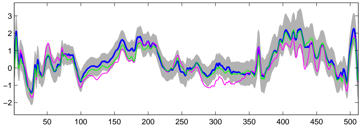
Estimated U_{26}(t) using R-WFMM: Normal data, run 3
