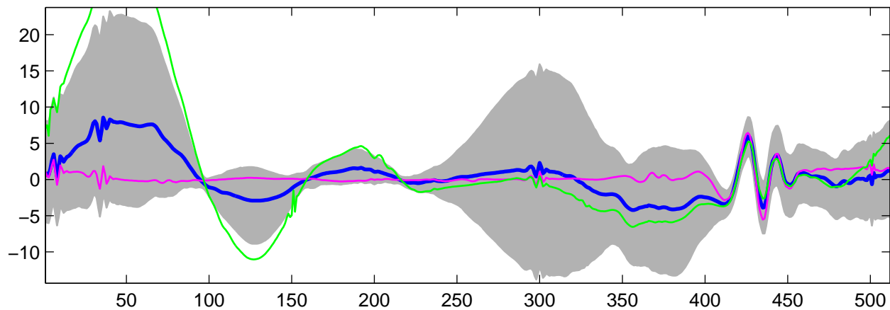
Estimated U_{26}(t) using G-WFMM: t_1 data, run 3
