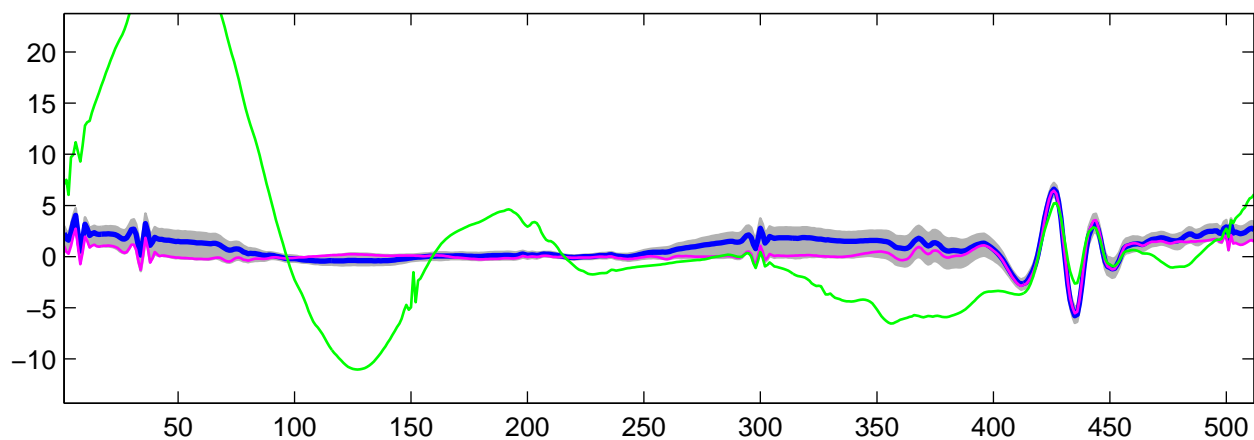
Estimated U_{26}(t) using R-WFMM: t_1 data, run 3
