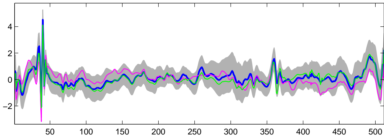
Estimated U_{26}(t) using G-WFMM: t_2 data, run 3
