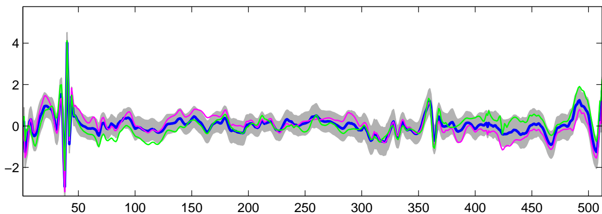
Estimated U_{26}(t) using R-WFMM: t_2 data, run 3
