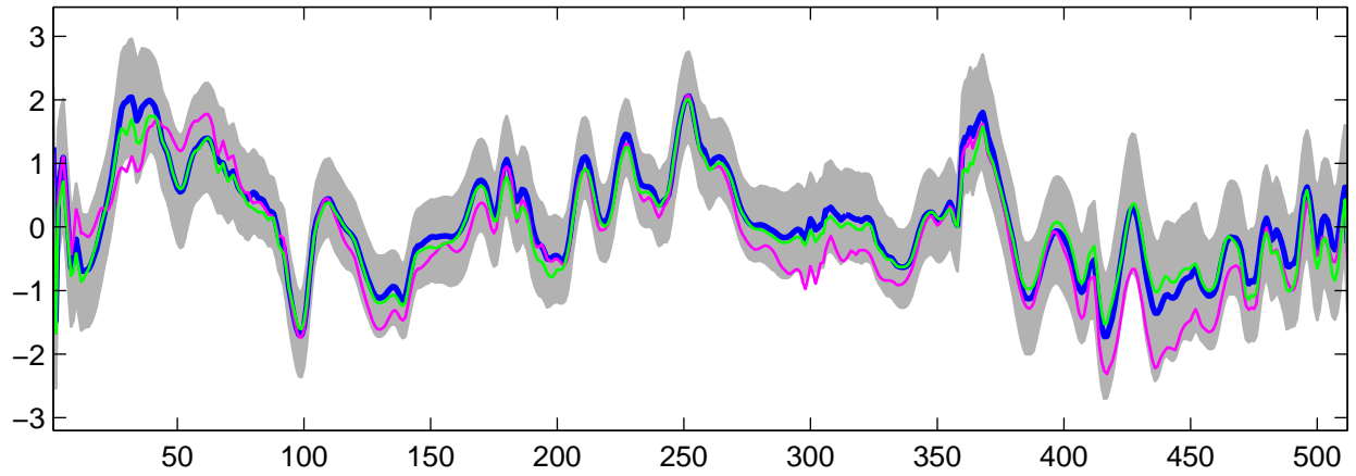
Estimated U_{27}(t) using G-WFMM: Normal data, run 3
