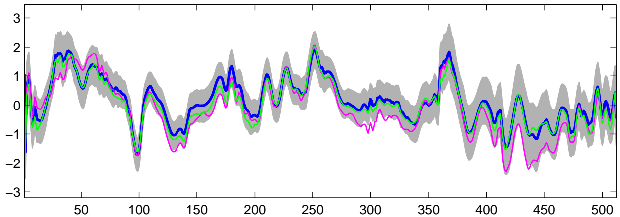
Estimated U_{27}(t) using R-WFMM: Normal data, run 3
