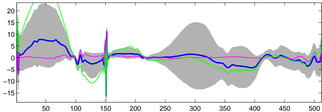
Estimated U_{27}(t) using G-WFMM: t_1 data, run 3
