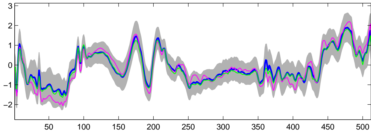
Estimated U_{27}(t) using G-WFMM: t_3 data, run 3
