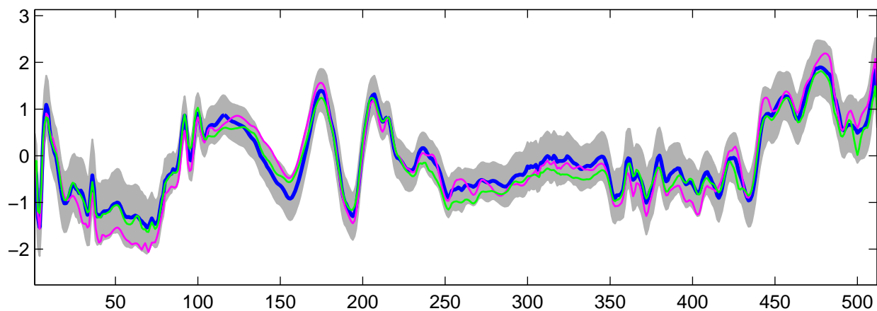
Estimated U_{27}(t) using R-WFMM: t_3 data, run 3
