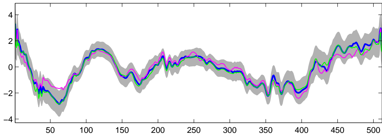
Estimated U_{28}(t) using G-WFMM: DE data, run 3
