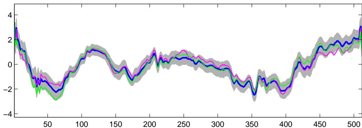
Estimated U_{28}(t) using R-WFMM: DE data, run 3
