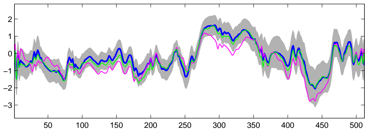
Estimated U_{28}(t) using R-WFMM: Normal data, run 3
