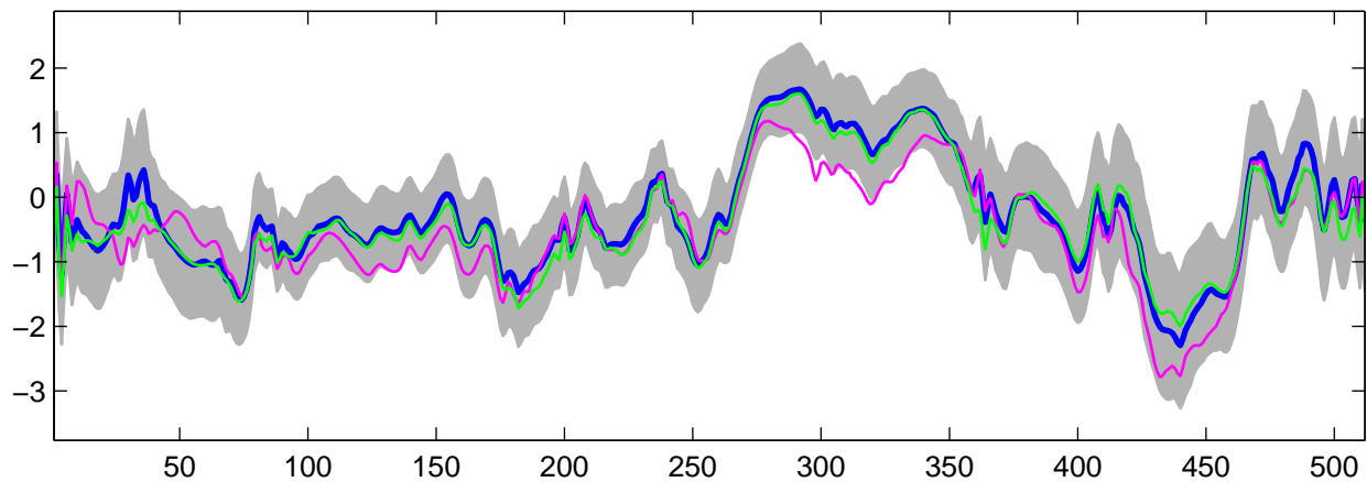
Estimated U_{28}(t) using G-WFMM: Normal data, run 3
