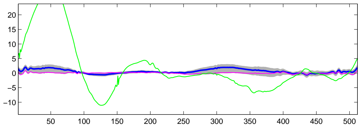
Estimated U_{28}(t) using R-WFMM: t_1 data, run 3
