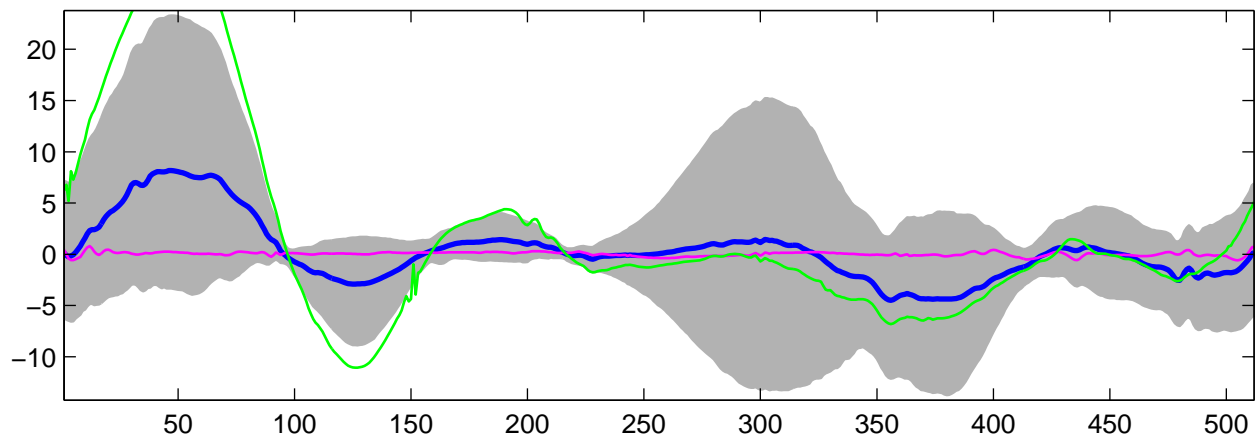
Estimated U_{28}(t) using G-WFMM: t_1 data, run 3
