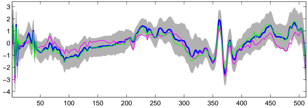
Estimated U_{28}(t) using G-WFMM: t_2 data, run 3
