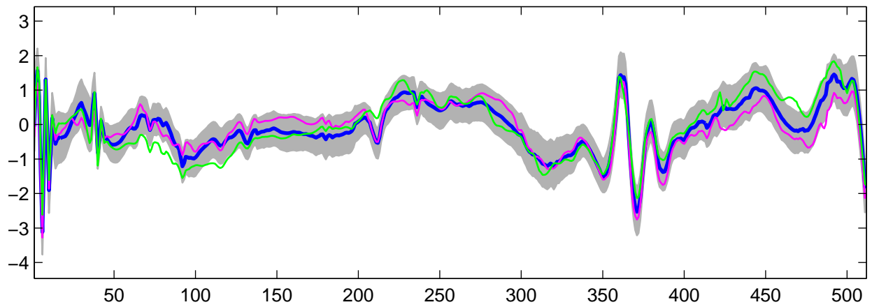
Estimated U_{28}(t) using R-WFMM: t_2 data, run 3
