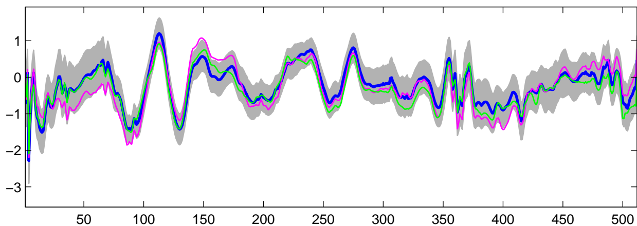
Estimated U_{28}(t) using R-WFMM: t_3 data, run 3
