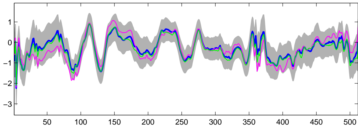
Estimated U_{28}(t) using G-WFMM: t_3 data, run 3
