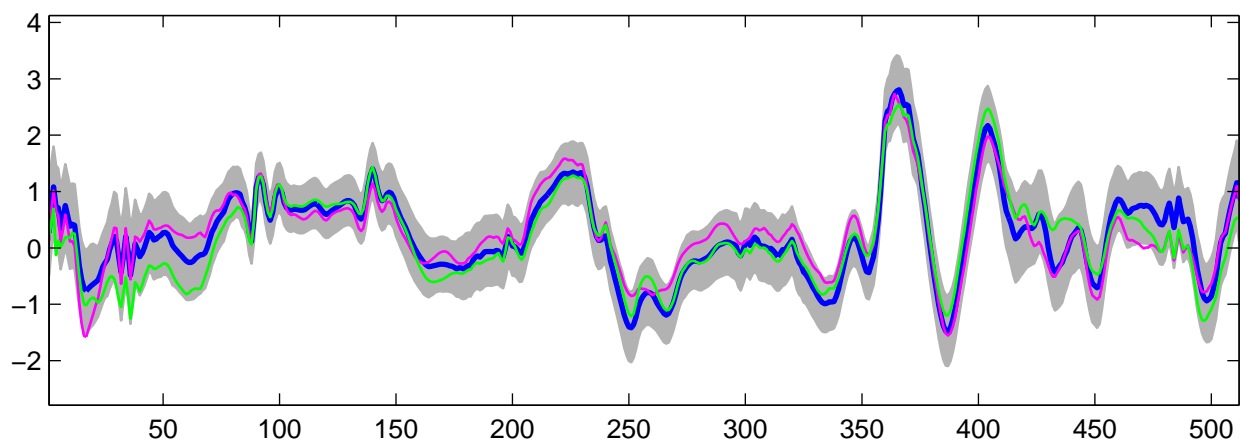
Estimated U_{29}(t) using R-WFMM: DE data, run 3
