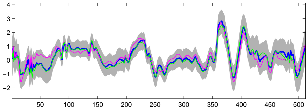
Estimated U_{29}(t) using G-WFMM: DE data, run 3
