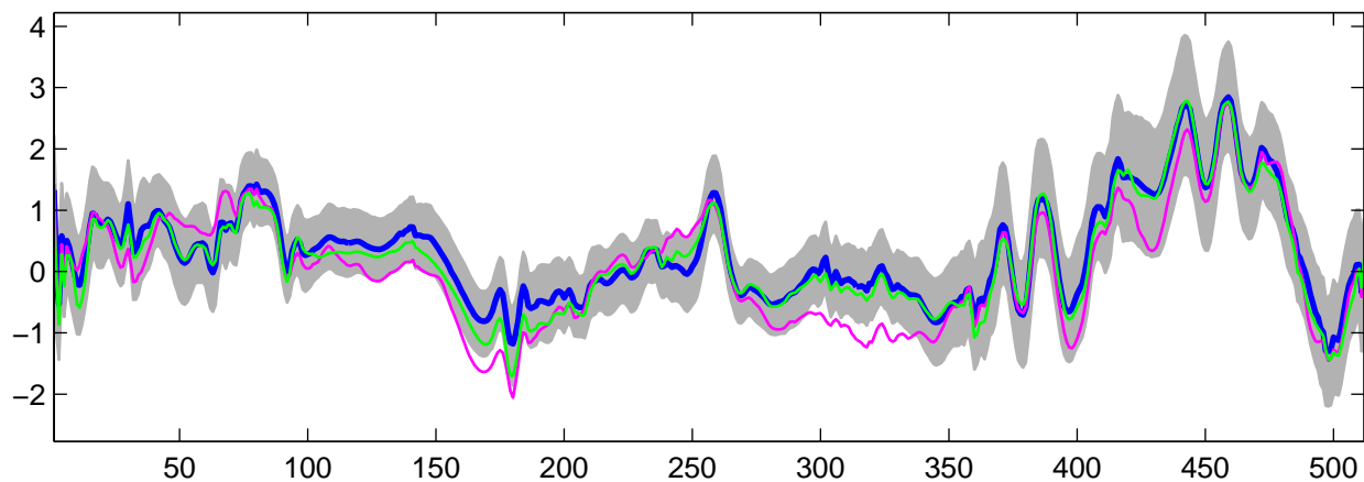
Estimated U_{29}(t) using R-WFMM: Normal data, run 3
