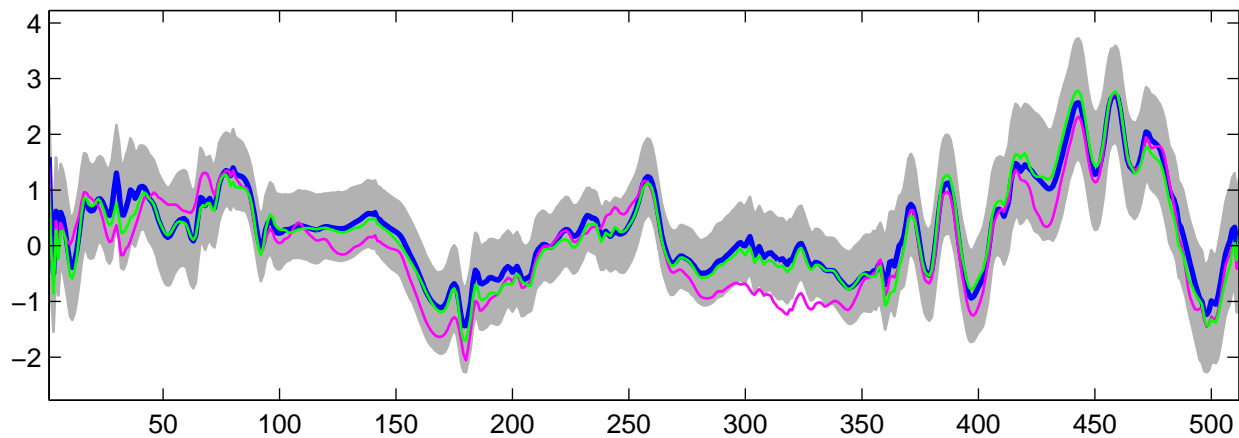
Estimated U_{29}(t) using G-WFMM: Normal data, run 3
