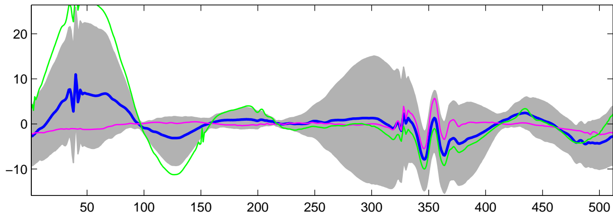
Estimated U_{29}(t) using G-WFMM: t_1 data, run 3
