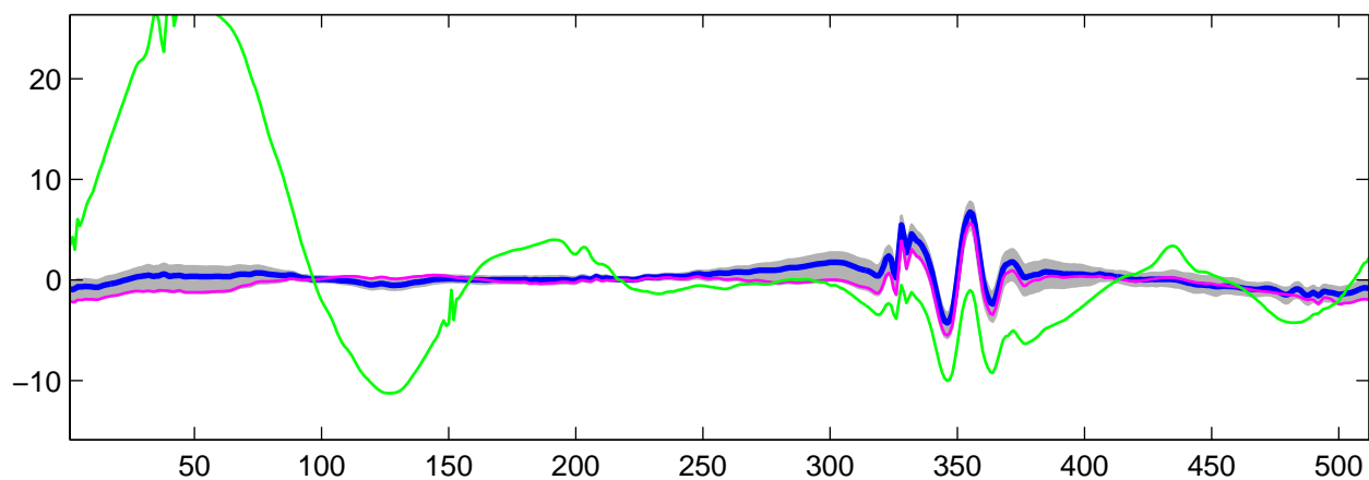
Estimated U_{29}(t) using R-WFMM: t_1 data, run 3
