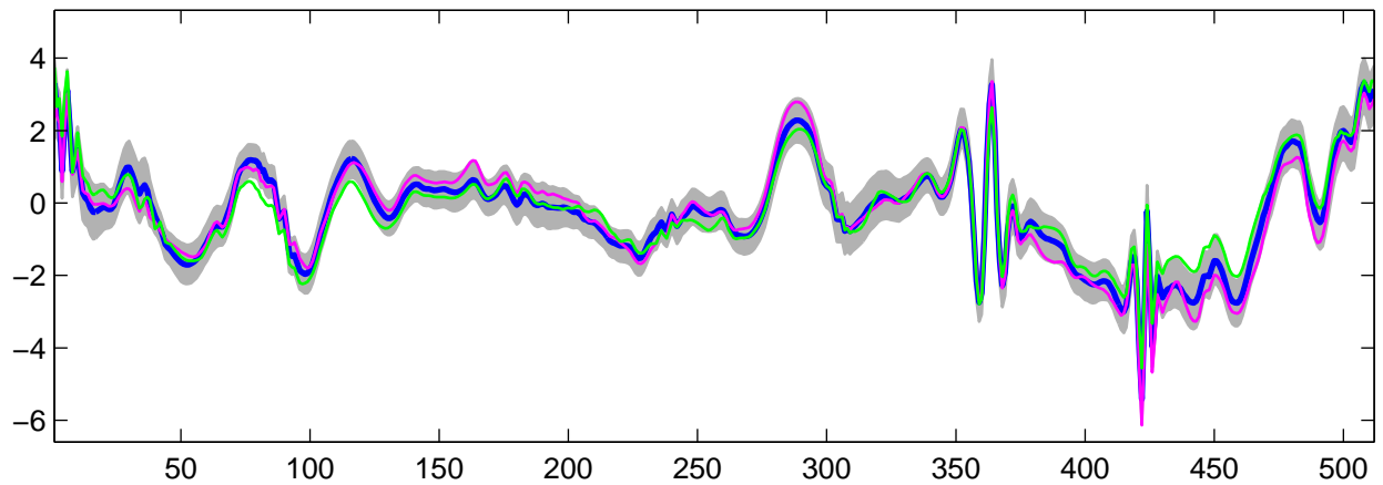
Estimated U_{29}(t) using R-WFMM: t_2 data, run 3
