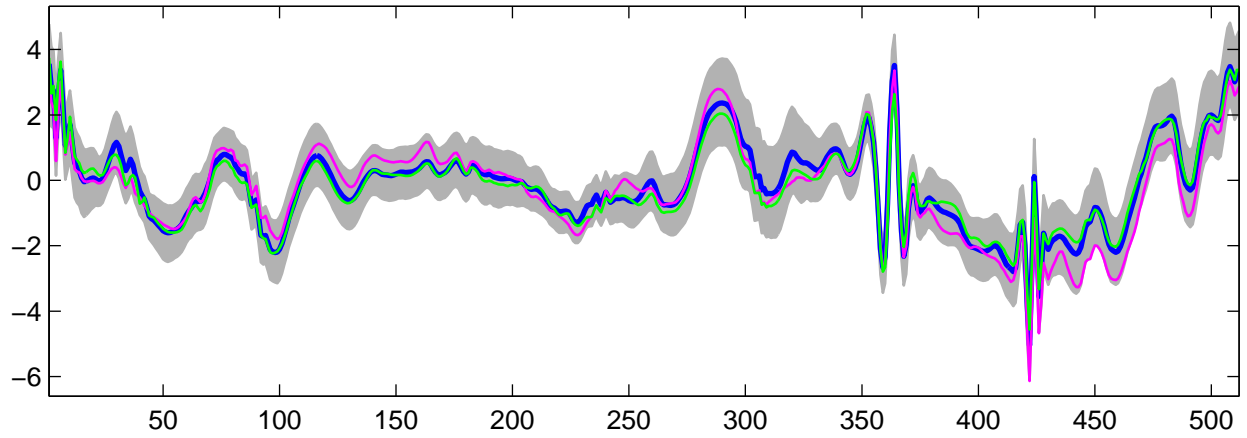
Estimated U_{29}(t) using G-WFMM: t_2 data, run 3
