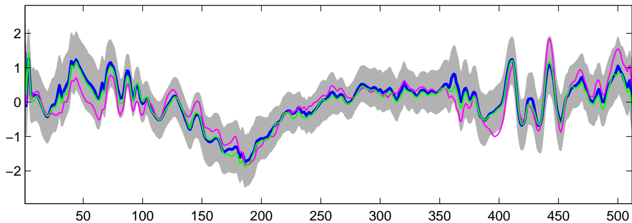
Estimated U_{29}(t) using G-WFMM: t_3 data, run 3
