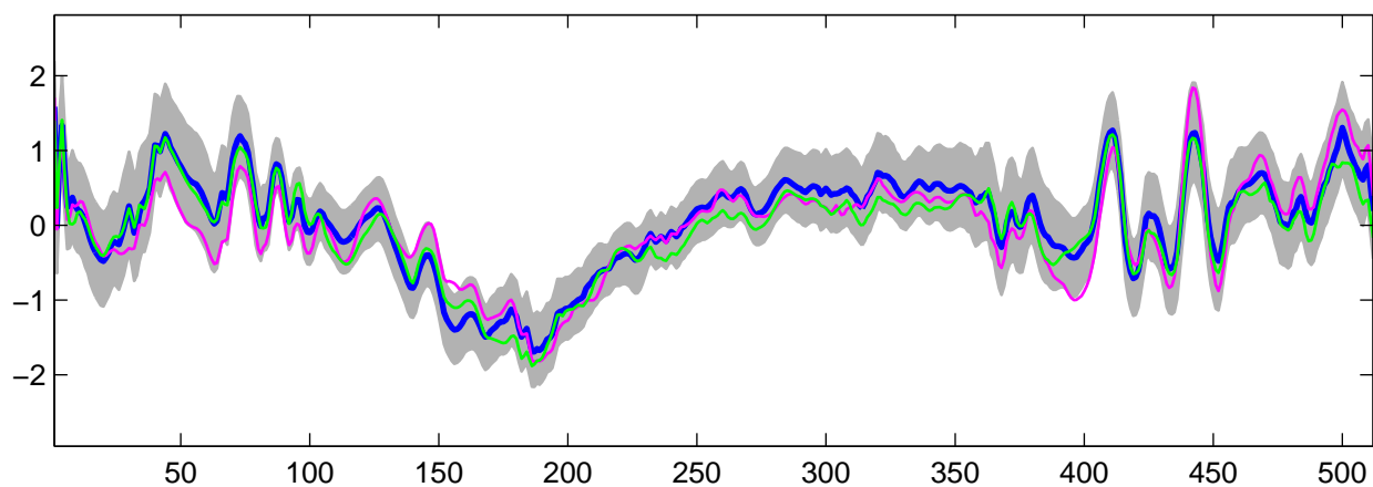
Estimated U_{29}(t) using R-WFMM: t_3 data, run 3
