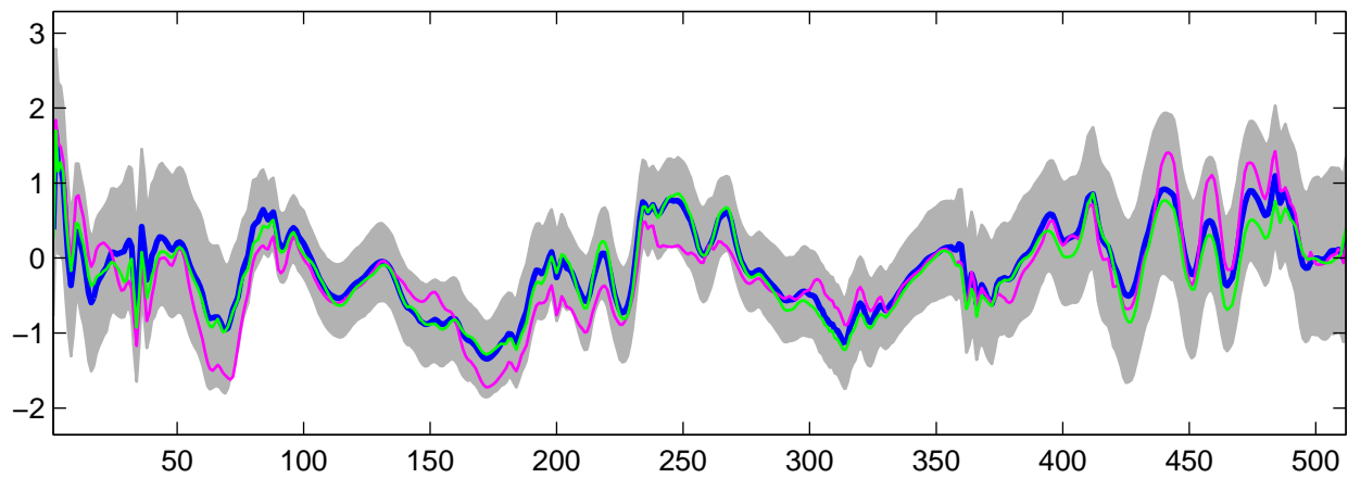
Estimated U_2(t) using G-WFMM: DE data, run 3
