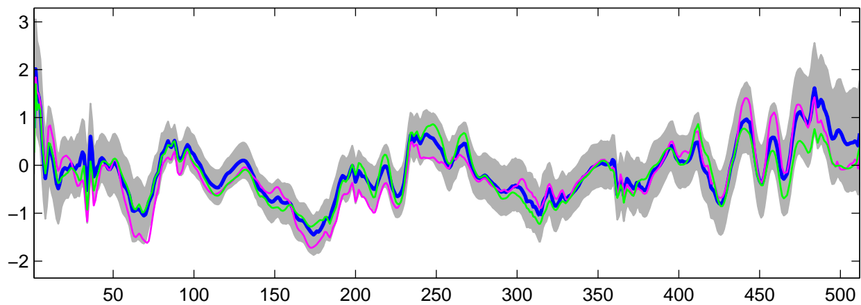
Estimated U_2(t) using R-WFMM: DE data, run 3
