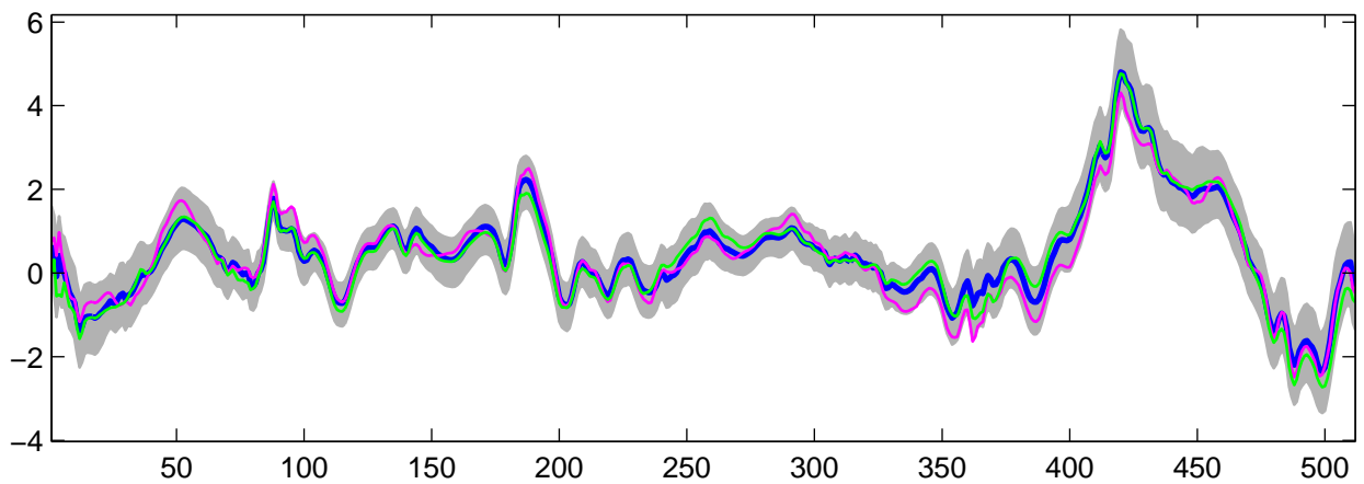
Estimated U_2(t) using R-WFMM: Normal data, run 3
