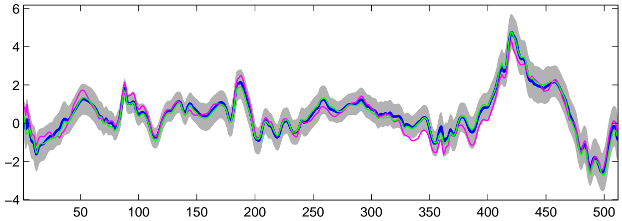
Estimated U_2(t) using G-WFMM: Normal data, run 3
