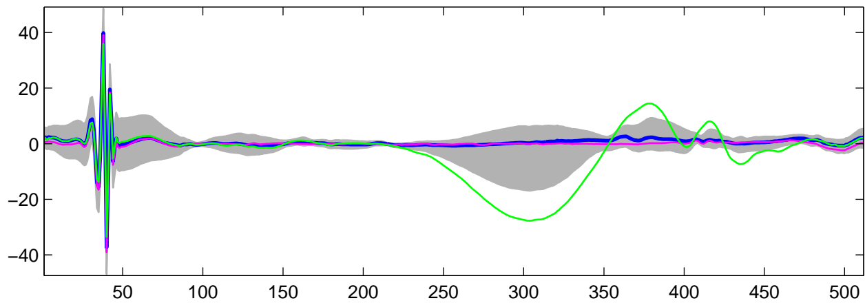
Estimated U_2(t) using G-WFMM: t_1 data, run 3
