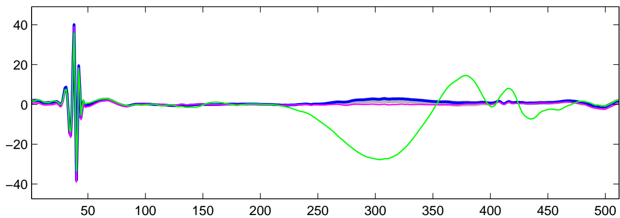
Estimated U_2(t) using R-WFMM: t_1 data, run 3
