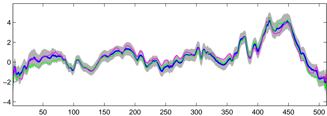
Estimated U_{30}(t) using R-WFMM: DE data, run 3
