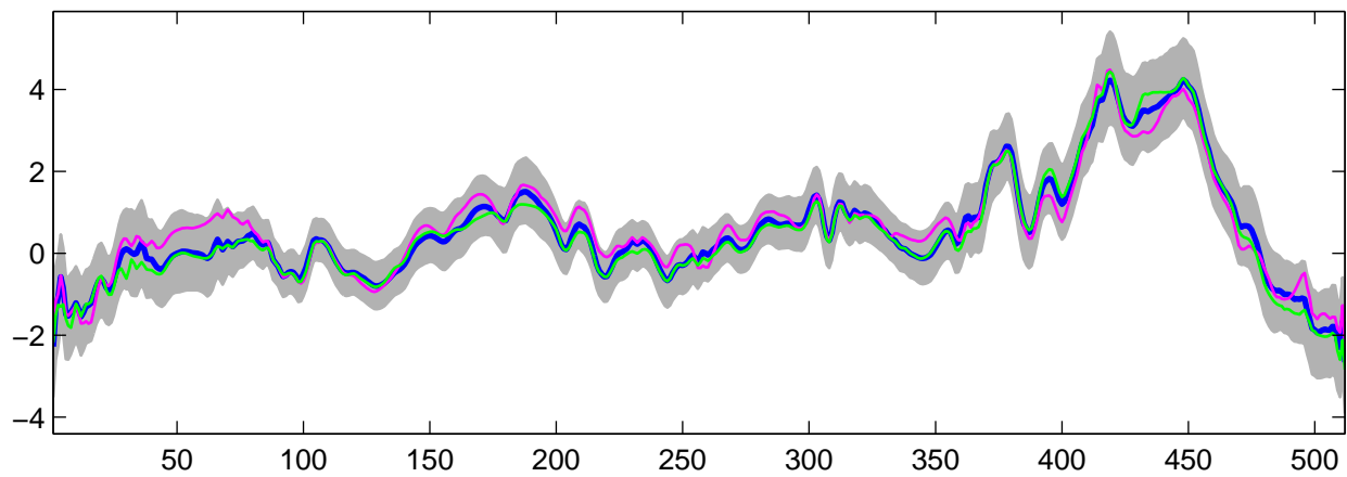
Estimated U_{30}(t) using G-WFMM: DE data, run 3
