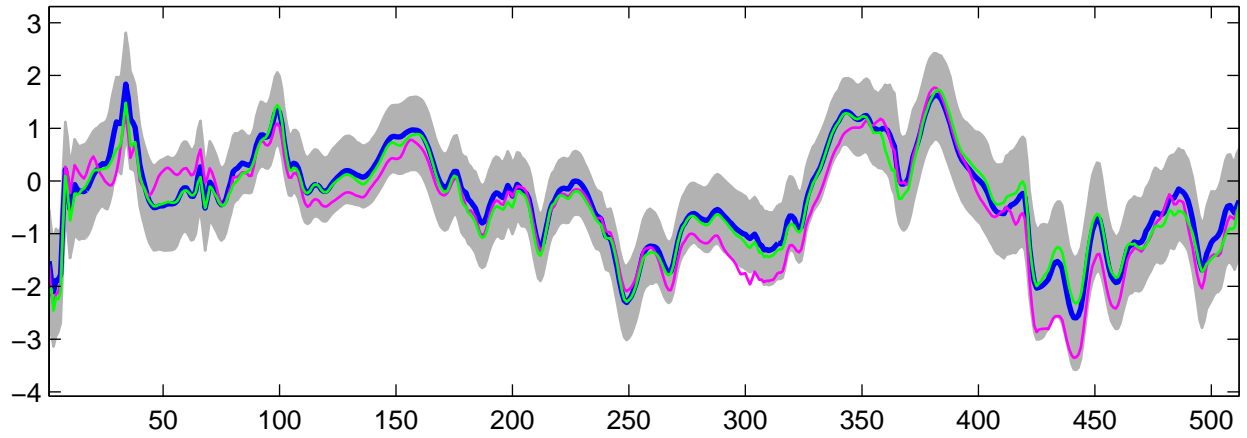
Estimated U_{30}(t) using G-WFMM: Normal data, run 3
