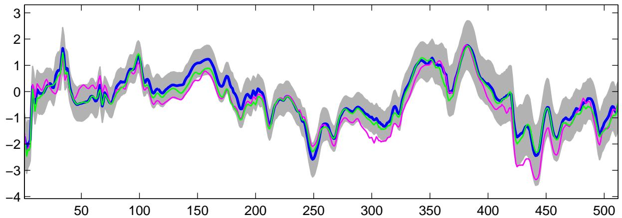
Estimated U_{30}(t) using R-WFMM: Normal data, run 3
