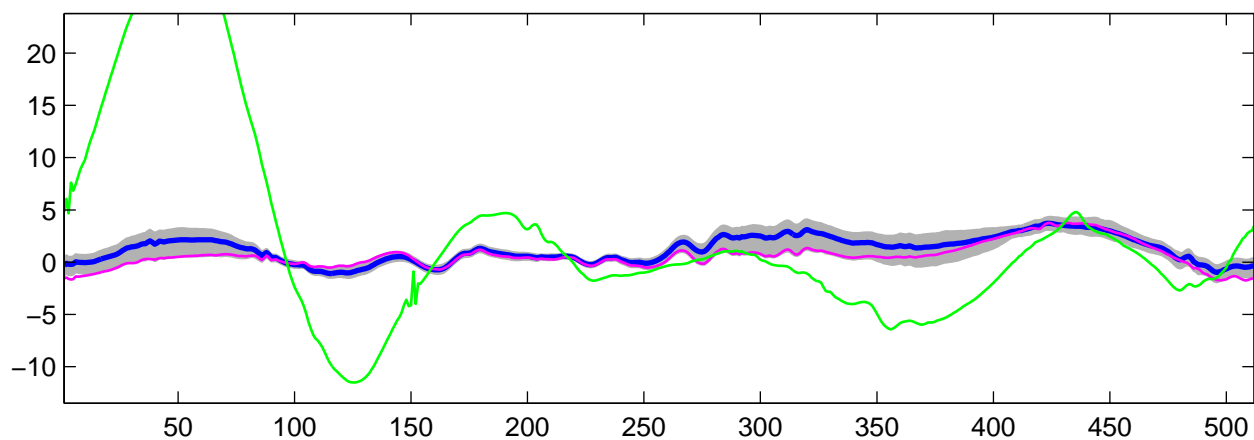
Estimated U_{30}(t) using R-WFMM: t_1 data, run 3
