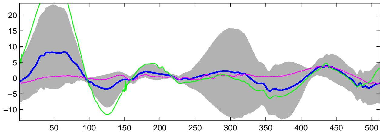
Estimated U_{30}(t) using G-WFMM: t_1 data, run 3
