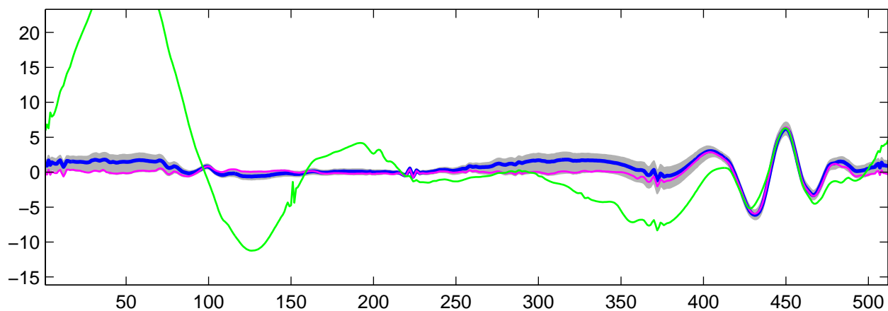
Estimated U_{31}(t) using R-WFMM: t_1 data, run 3
