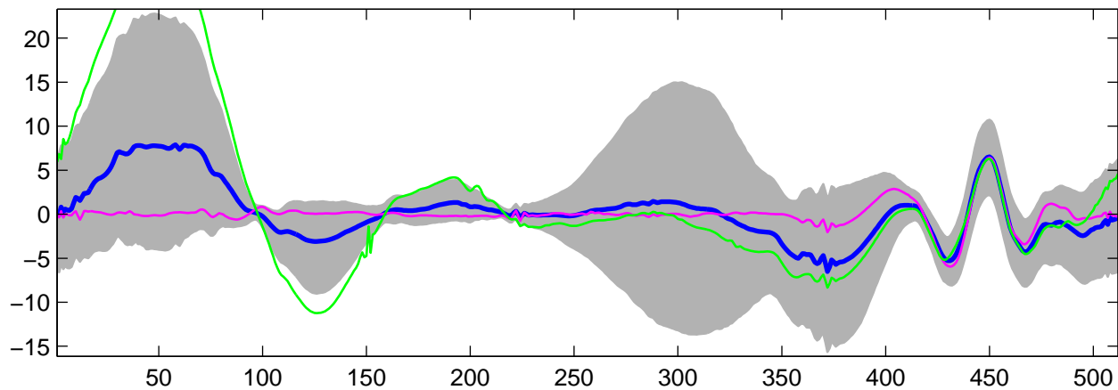
Estimated U_{31}(t) using G-WFMM: t_1 data, run 3
