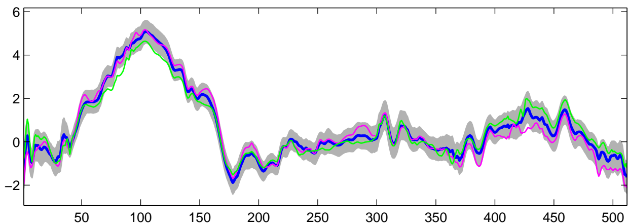
Estimated U_{31}(t) using R-WFMM: t_2 data, run 3
