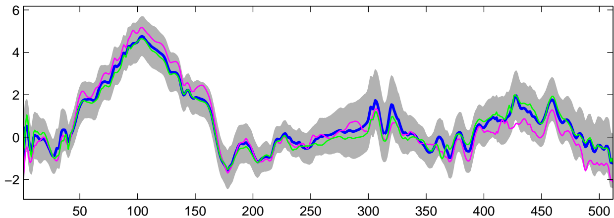
Estimated U_{31}(t) using G-WFMM: t_2 data, run 3
