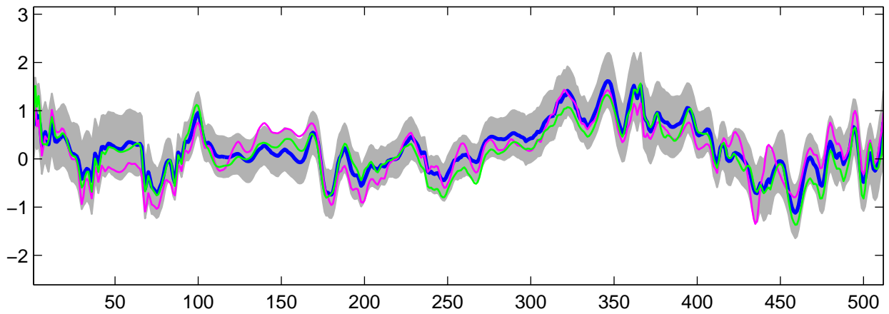
Estimated U_{31}(t) using R-WFMM: t_3 data, run 3
