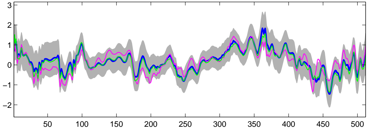
Estimated U_{31}(t) using G-WFMM: t_3 data, run 3
