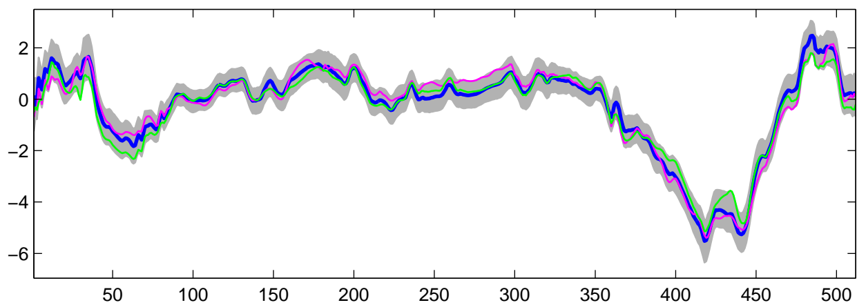
Estimated U_{32}(t) using R-WFMM: DE data, run 3
