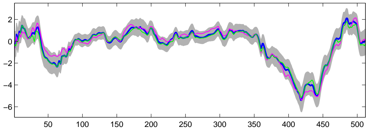
Estimated U_{32}(t) using G-WFMM: DE data, run 3
