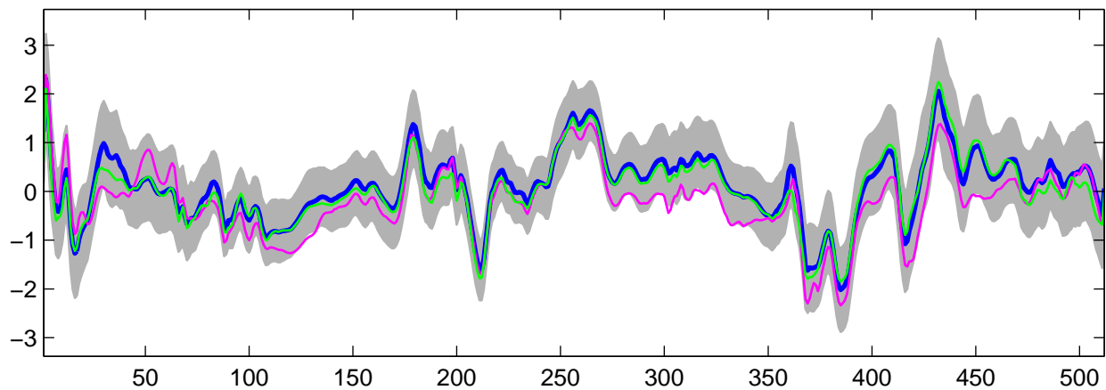
Estimated U_{32}(t) using G-WFMM: Normal data, run 3
