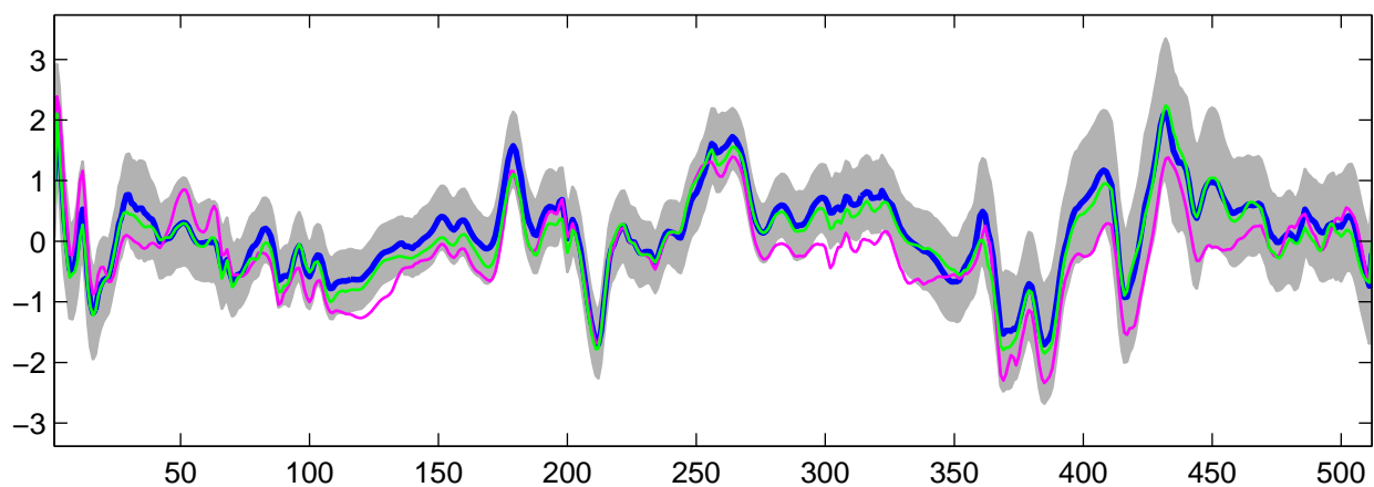
Estimated U_{32}(t) using R-WFMM: Normal data, run 3
