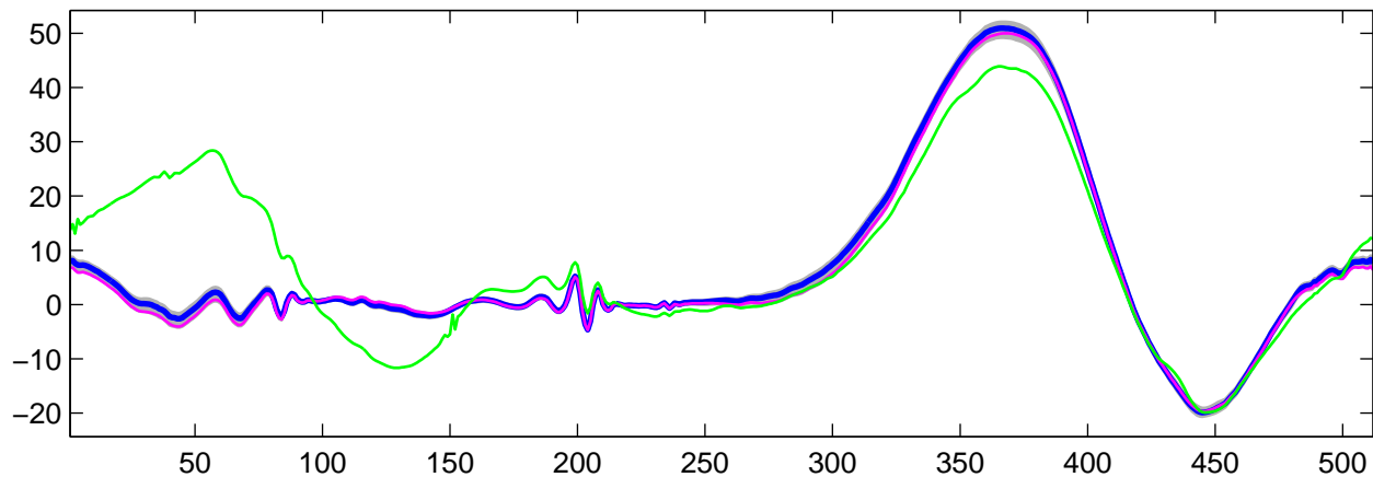
Estimated U_{32}(t) using R-WFMM: t_1 data, run 3
