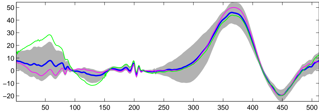
Estimated U_{32}(t) using G-WFMM: t_1 data, run 3
