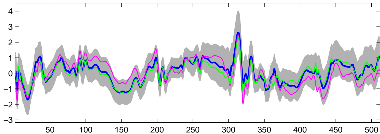
Estimated U_{32}(t) using G-WFMM: t_2 data, run 3
