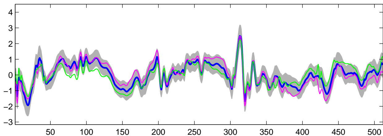
Estimated U_{32}(t) using R-WFMM: t_2 data, run 3
