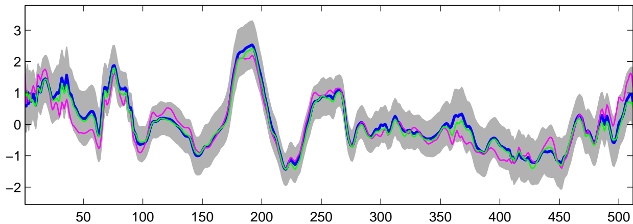
Estimated U_{32}(t) using G-WFMM: t_3 data, run 3
