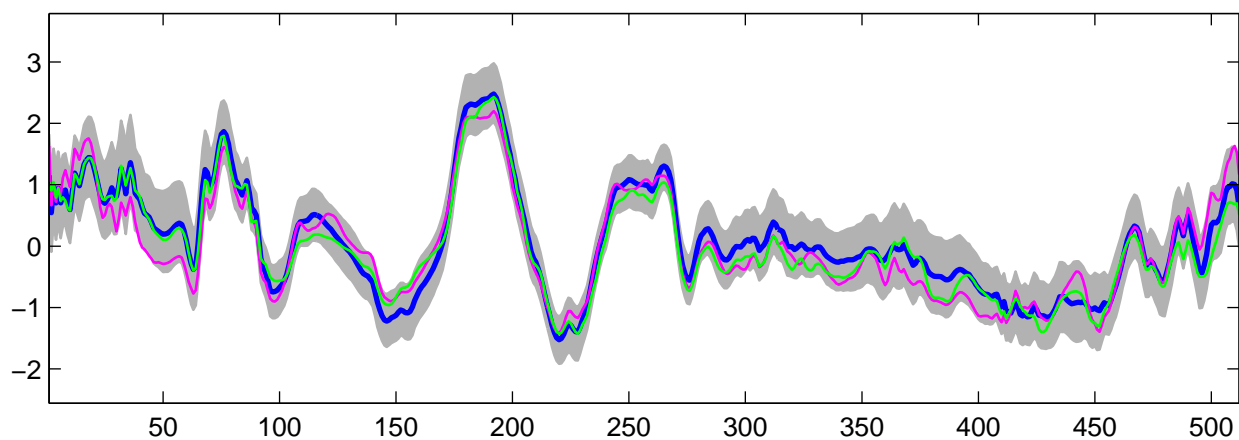
Estimated U_{32}(t) using R-WFMM: t_3 data, run 3
