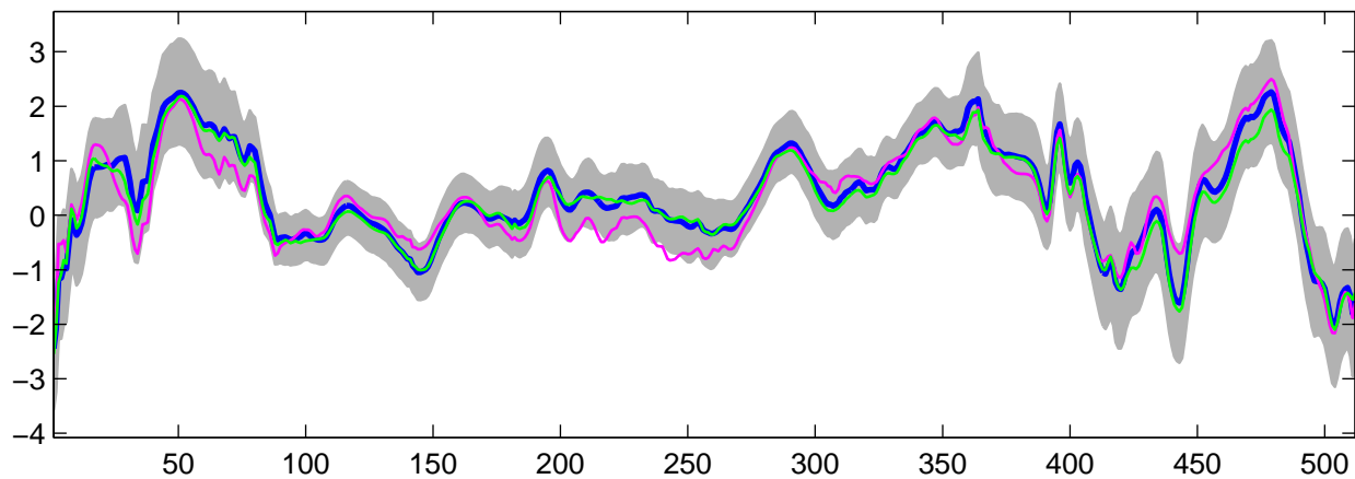
Estimated U_3(t) using G-WFMM: DE data, run 3
