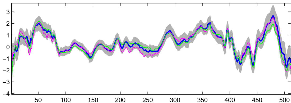
Estimated U_3(t) using R-WFMM: DE data, run 3
