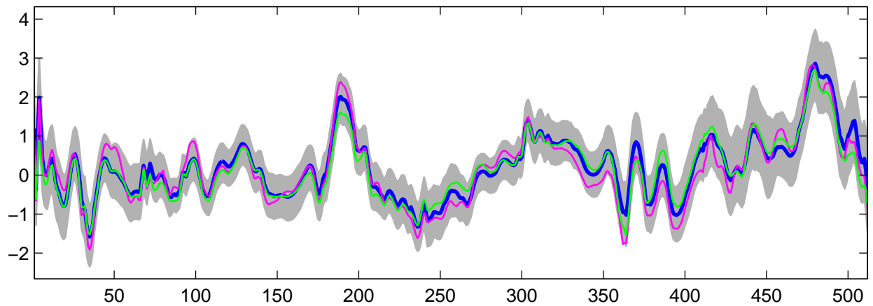
Estimated U_3(t) using R-WFMM: Normal data, run 3
