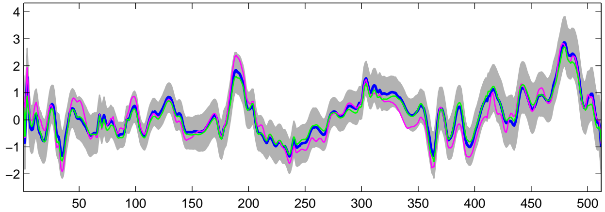
Estimated U_3(t) using G-WFMM: Normal data, run 3
