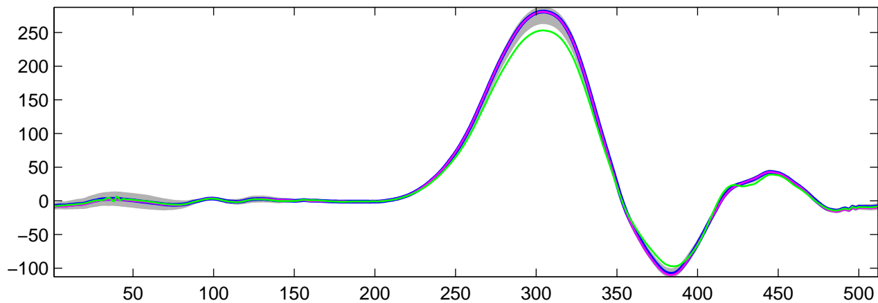
Estimated U_3(t) using G-WFMM: t_1 data, run 3
