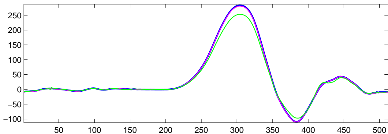
Estimated U_3(t) using R-WFMM: t_1 data, run 3
