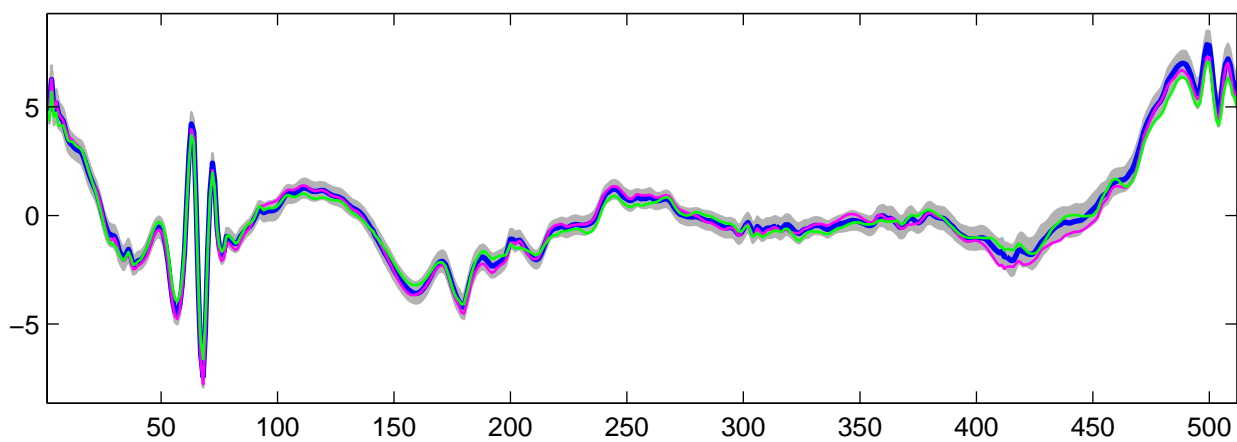
Estimated U_3(t) using R-WFMM: t_2 data, run 3
