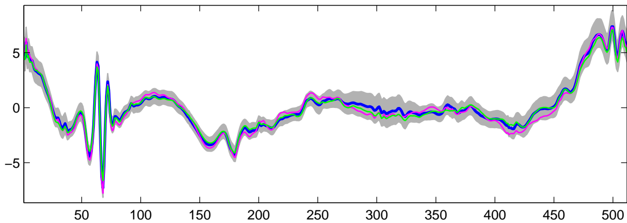
Estimated U_3(t) using G-WFMM: t_2 data, run 3
