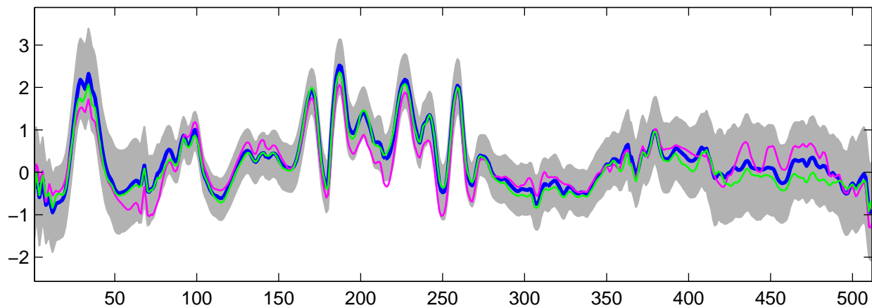
Estimated U_4(t) using G-WFMM: DE data, run 3
