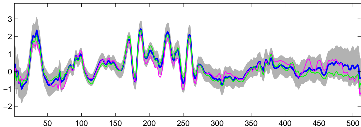
Estimated U_4(t) using R-WFMM: DE data, run 3
