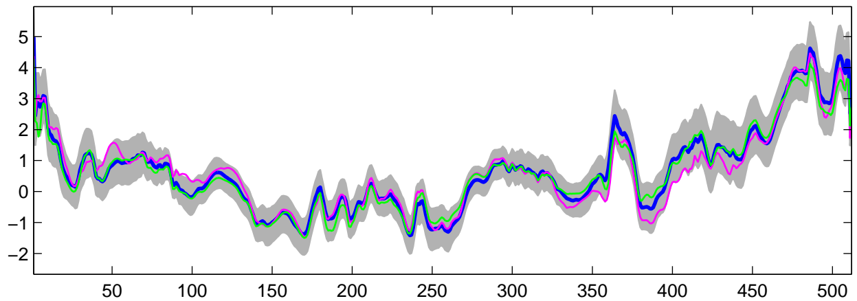
Estimated U_4(t) using R-WFMM: Normal data, run 3
