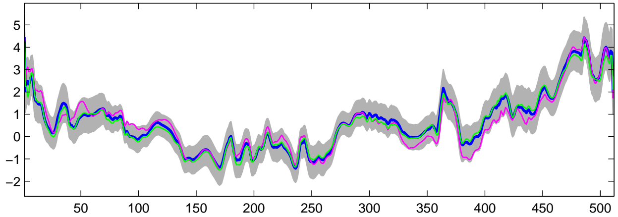
Estimated U_4(t) using G-WFMM: Normal data, run 3
